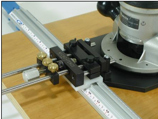
Single Clamp Interface
